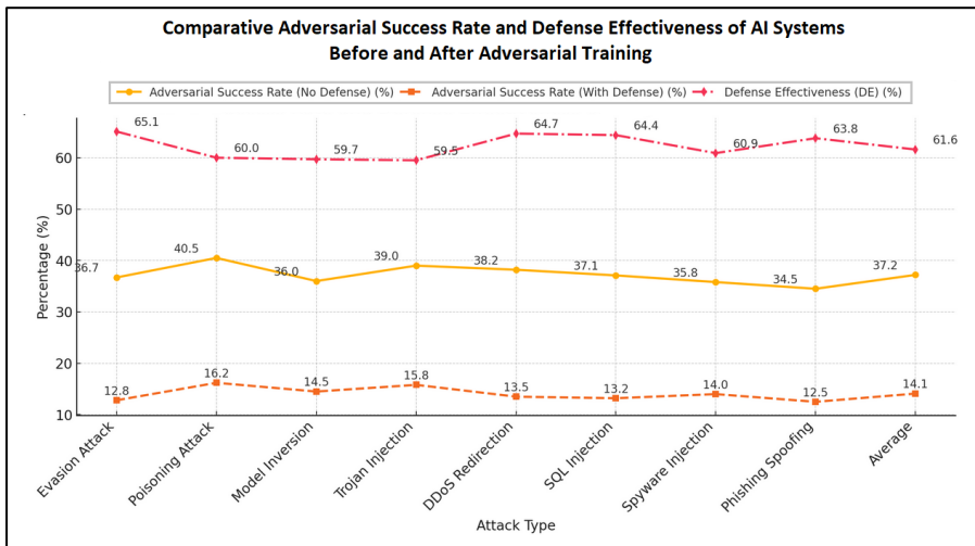
Figure 4. Comparative Analysis of Adversarial Success Rates and Defense Effectiveness Across Multiple Attack Types with Impact of Adversarial Training on AI Systems
